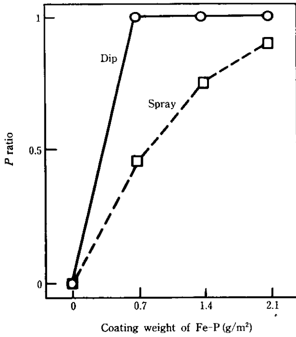
Fig. 11 Effect of Fe-P upper coating weight on wet adhesion of double layered Zn-Ni alloy electroplated steel
