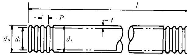
Fig. 2 Configuration of corrugated stainless steel tube
