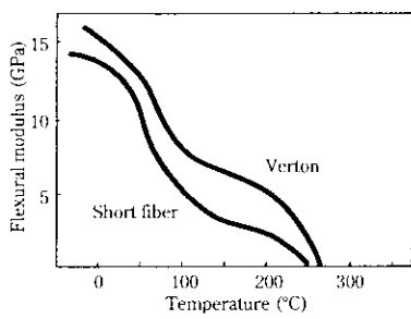
Fig. 2 Flexural modulus of nylon Verton and short fiber/nylon
